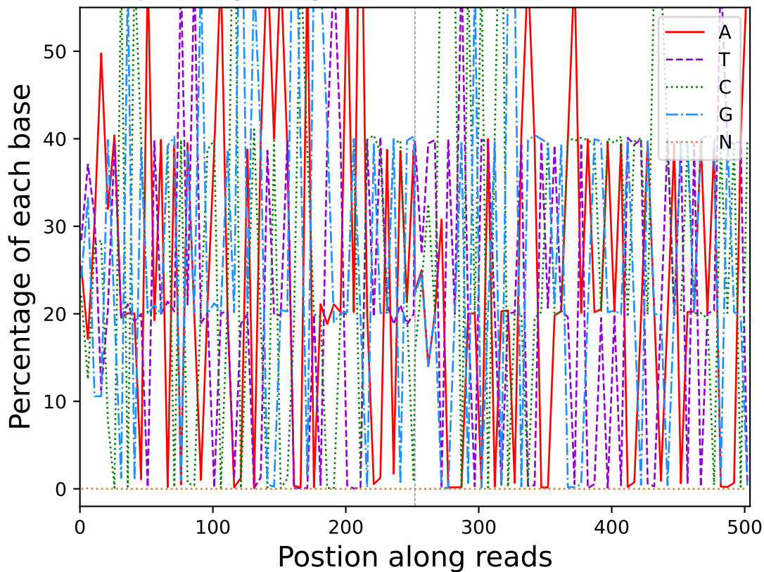
Base percentage along reads (R10710)
